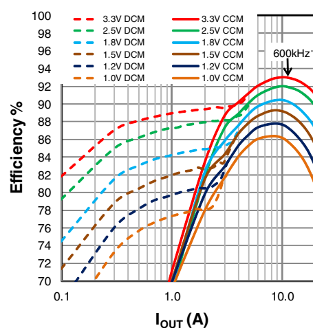
Figure 21: Efficiency, V_{\text{IN}}=12\text{V}
