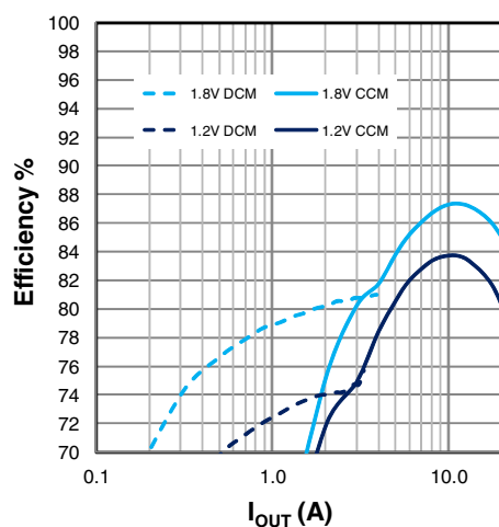
Figure 23: Efficiency, V_{\text{IN}}=19.6\text{V}
