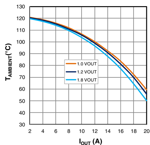
Figure 20: Maximum T_{\text{AMBIENT}} vs I_{\text{OUT}} , V_{\text{IN}}=5\text{V}
