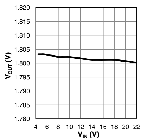
Figure 2: Line regulation
