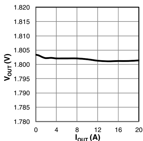
Figure 1: Load Regulation
