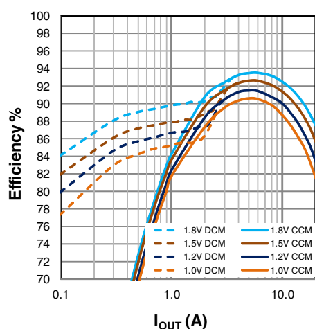
Figure 19: Efficiency, V_{\text{IN}}=5\text{V}
