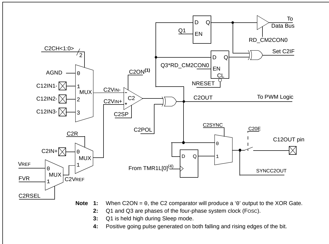
FIGURE 18-3: COMPARATOR C2 SIMPLIFIED BLOCK DIAGRAM
