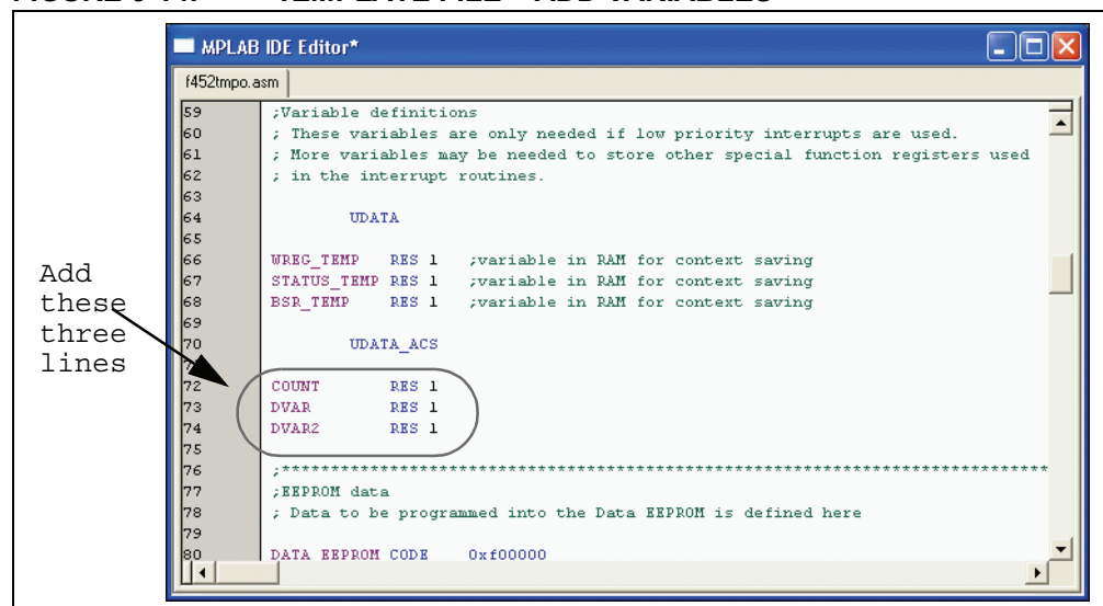
FIGURE 3-14: TEMPLATE FILE – ADD VARIABLES
