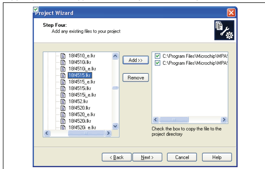
FIGURE 3-7: PROJECT WIZARD – SELECT LINKER SCRIPT
