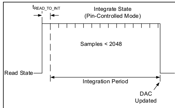
FIGURE 4-7: Pin Controlled Integration Period.
