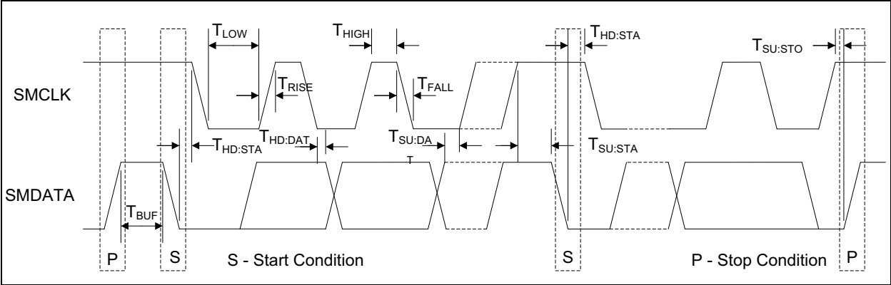
FIGURE 1-1: SMBus Timing.
