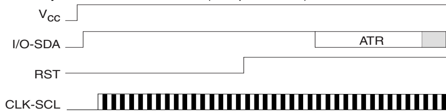
Figure 7. Asynchronous T = 0 Protocol (Gemplus Patent)
