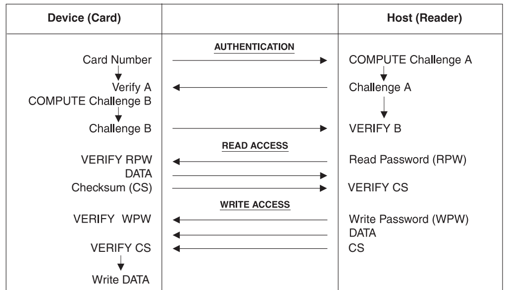
Figure 9. Password and Authentication Operations
