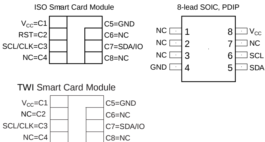
Figure 1. Package Configuration
