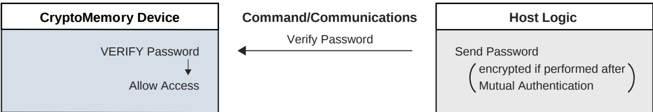
Figure 3. Password Verification
