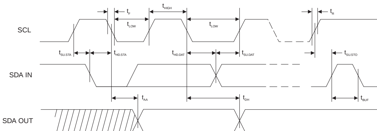
Figure 31. Bus Timing
