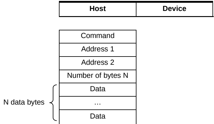
Figure 12. Write User Zone Command Functional Description
