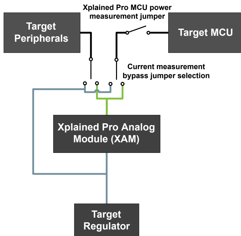
Figure 4-1 SAM L21 Xplained Pro XAM Implementation Block Diagram
