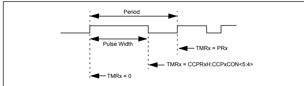
FIGURE 3-8: PWM ANALYSIS
