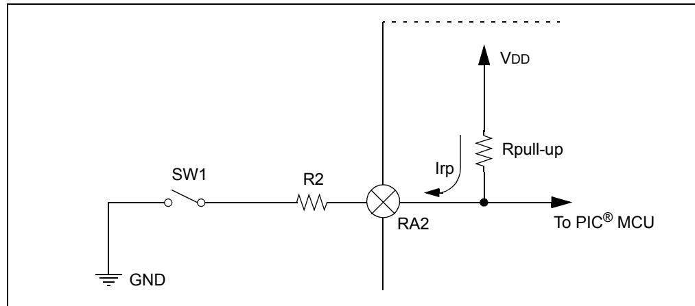
FIGURE 3-12: WEAK PULL-UP DIAGRAM
