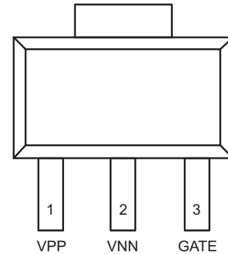
3-Lead SOT-223 (Top View)
