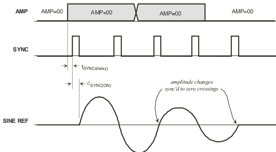
Figure 4: AMP Timing
