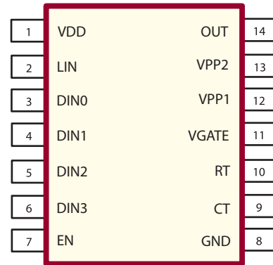
HV7100 (top view)
