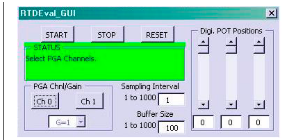
FIGURE 2-6: Hardware Status
