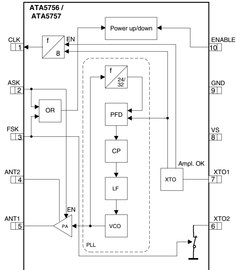
Figure 2-2. Block Diagram
