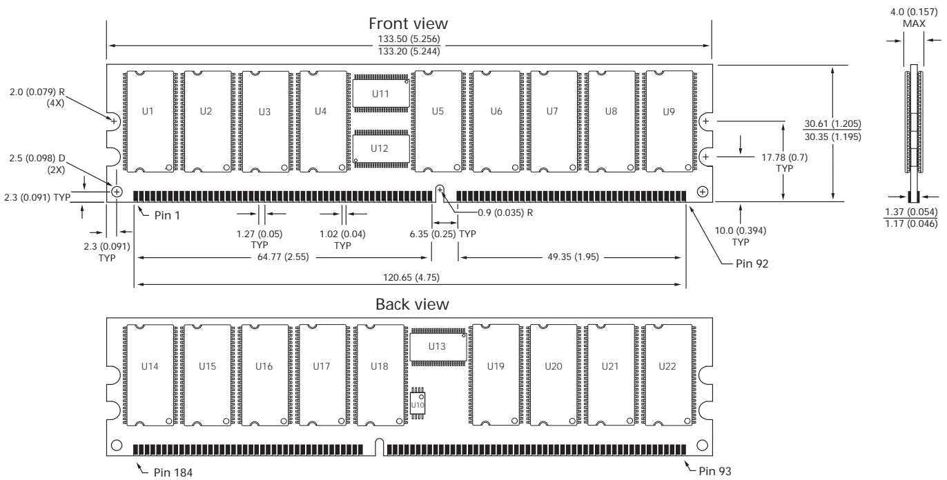
Figure 5: 184-Pin RDIMM Low-Profile Height
