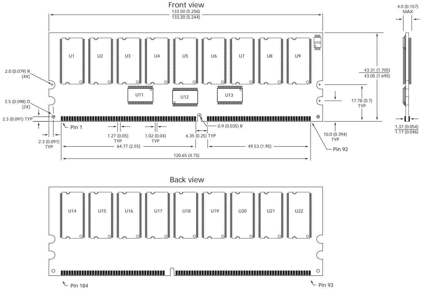
Figure 4: 184-Pin RDIMM Standard Height
