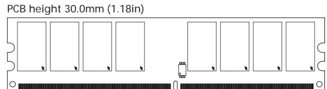
Figure 1: 240-Pin DIMM (MO-237 R/C A)
