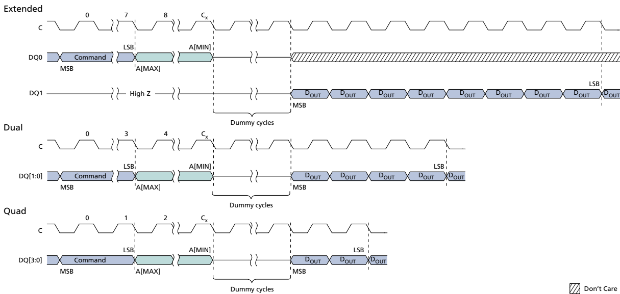
Figure 33: READ OTP Command
