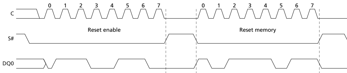
Figure 32: RESET ENABLE and RESET MEMORY Command
