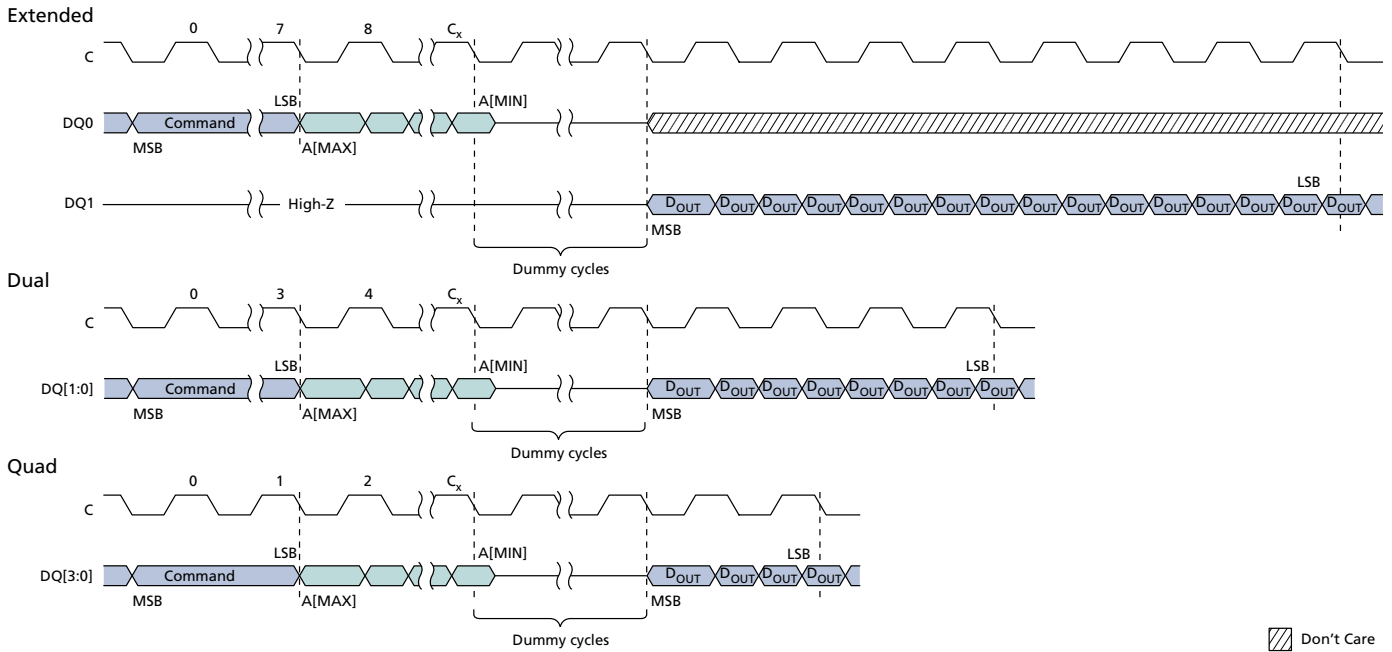
Figure 19: FAST READ Command – DTR
