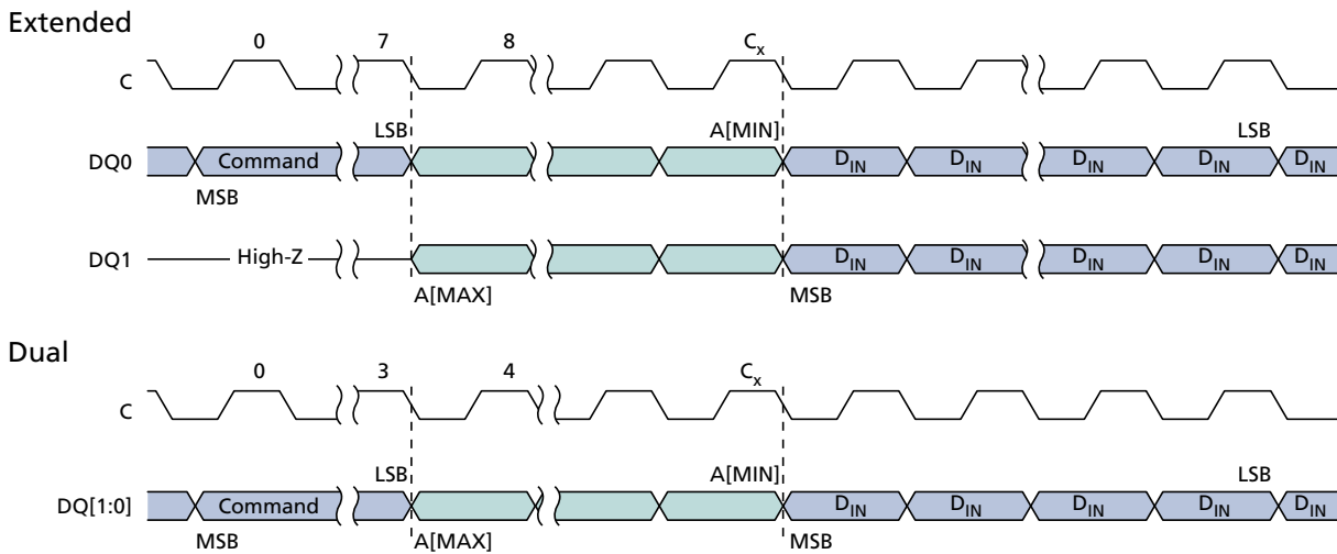
Figure 26: EXTENDED DUAL INPUT FAST PROGRAM Command
