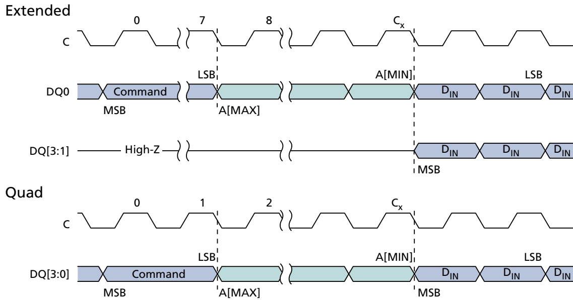
Figure 27: QUAD INPUT FAST PROGRAM Command
