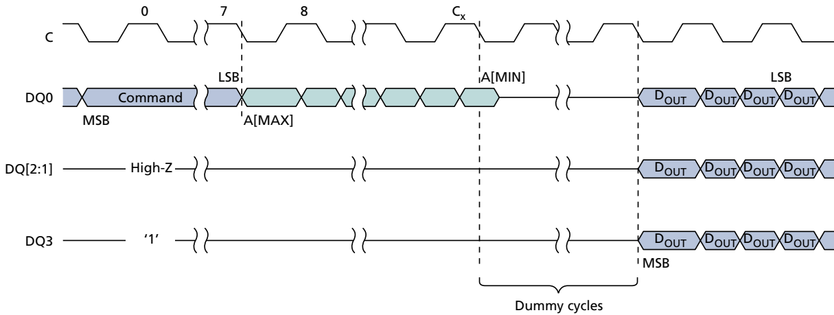
Figure 22: QUAD OUTPUT FAST READ Command – DTR
