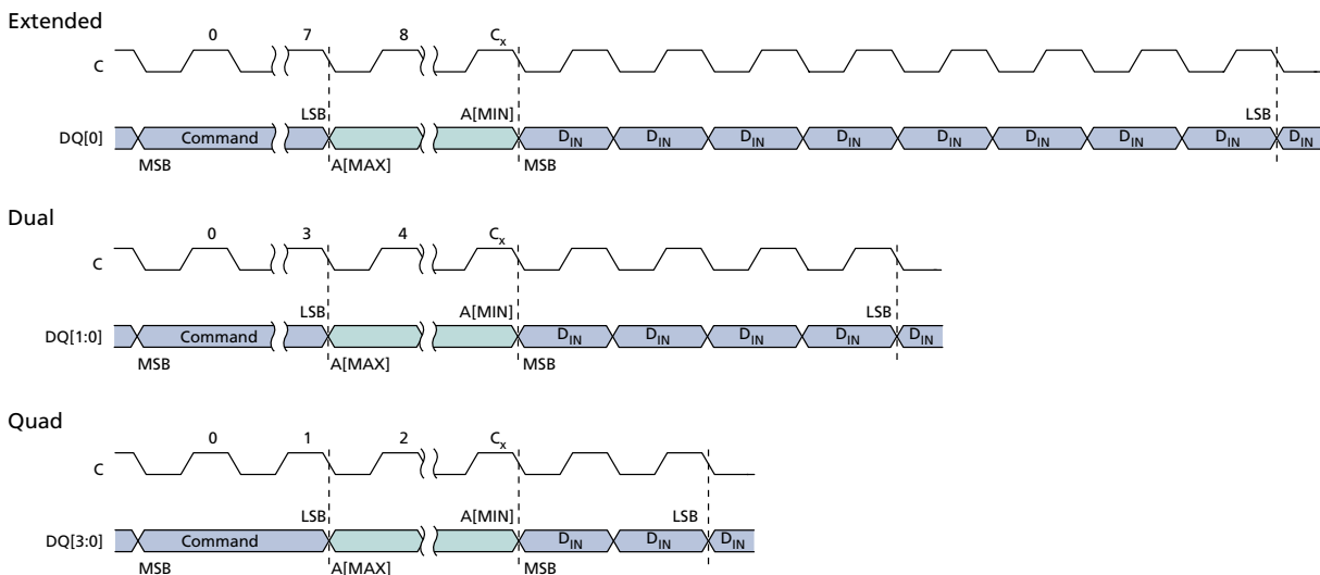
Figure 34: PROGRAM OTP Command
