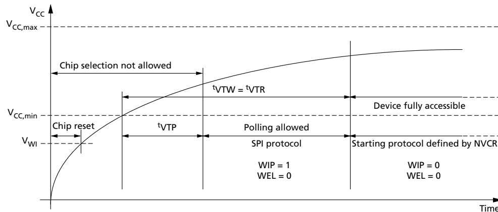
Figure 36: Power-Up Timing
