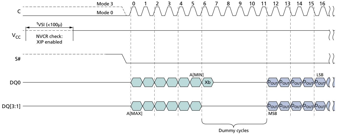
Figure 35: XIP Mode Directly After Power-On
