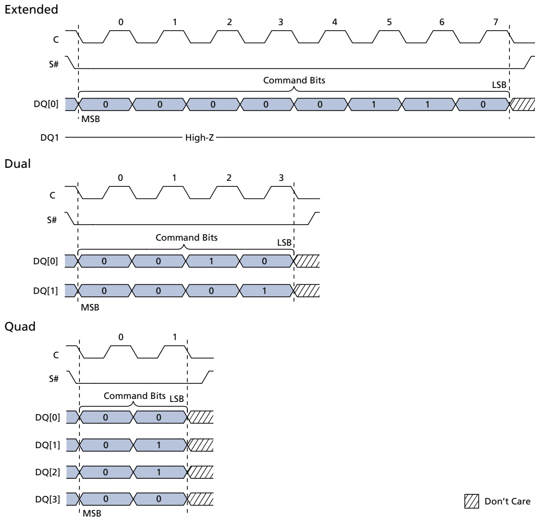
Figure 29: WRITE ENABLE and WRITE DISABLE Command Sequence
