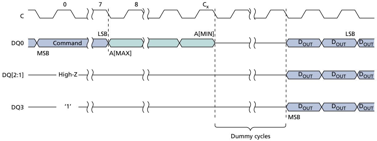
Figure 17: QUAD OUTPUT FAST READ Command
