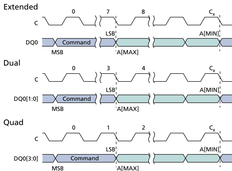
Figure 30: SUBSECTOR and SECTOR ERASE Command
