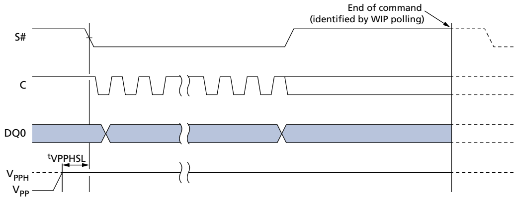
Figure 42: V PPH Timing
