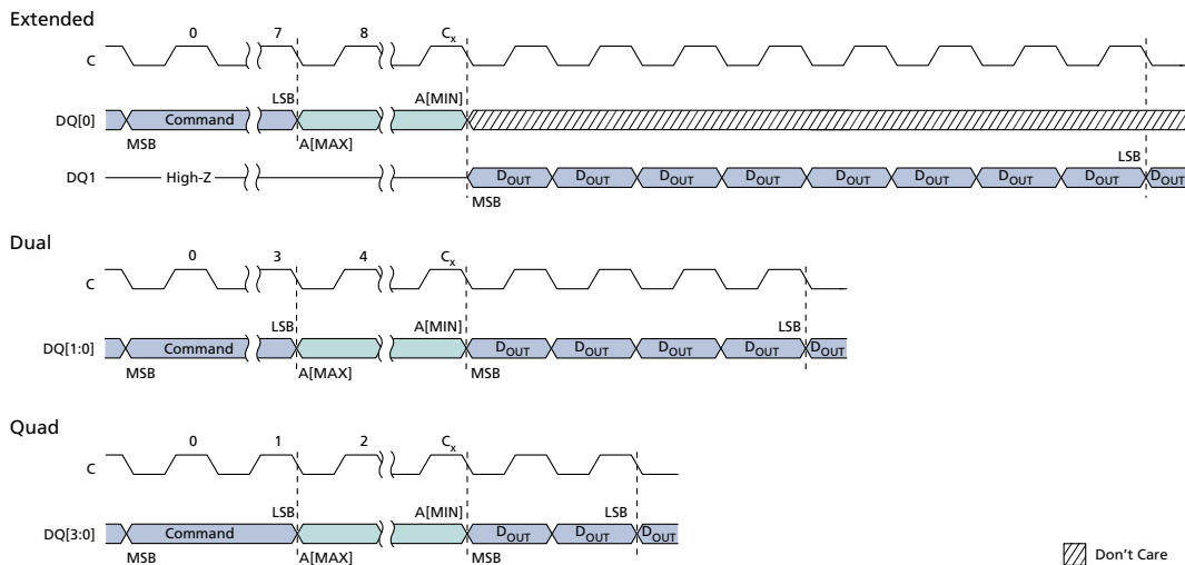
Figure 10: READ LOCK REGISTER Command
