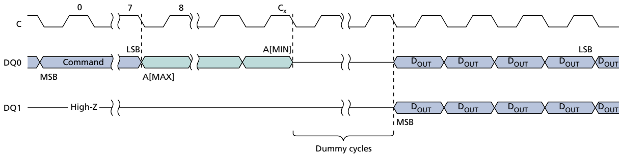
Figure 15: DUAL OUTPUT FAST READ Command
