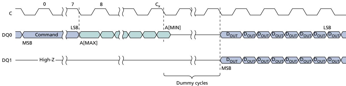
Figure 20: DUAL OUTPUT FAST READ Command – DTR
