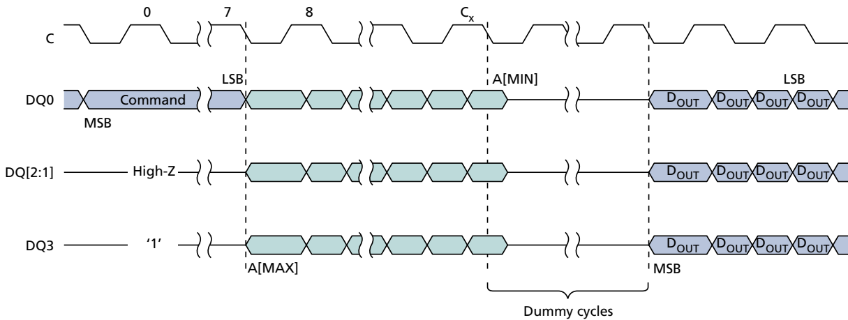
Figure 23: QUAD INPUT/OUTPUT FAST READ Command – DTR
