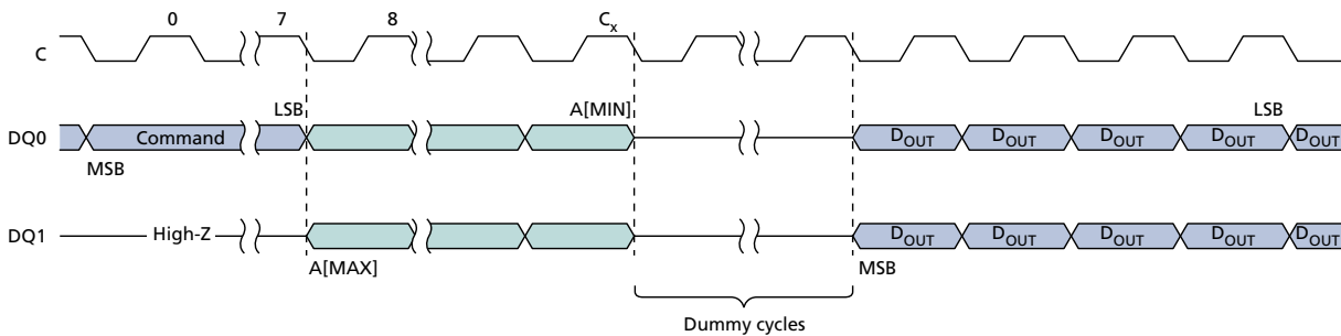
Figure 16: DUAL INPUT/OUTPUT FAST READ Command
