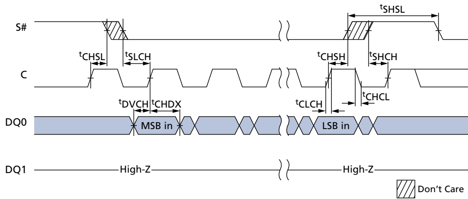
Figure 39: Serial Input Timing
