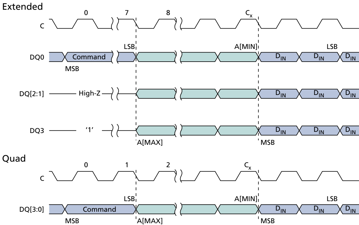
Figure 28: EXTENDED QUAD INPUT FAST PROGRAM Command
