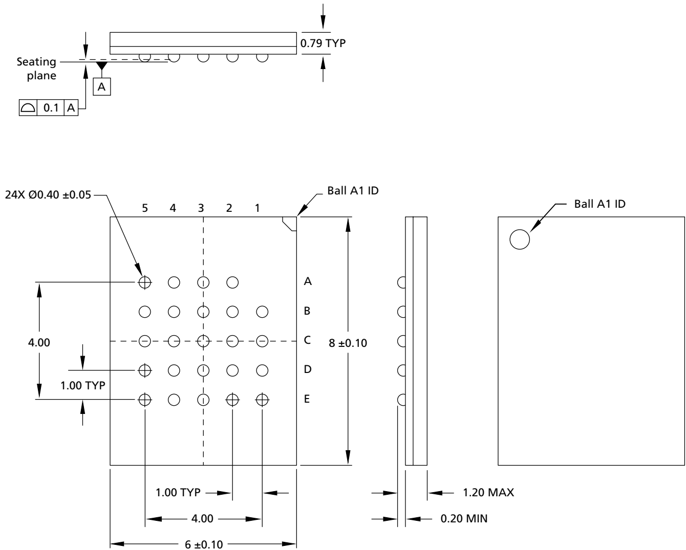
Figure 44: T-PBGA-24b05/6mm x 8mm
