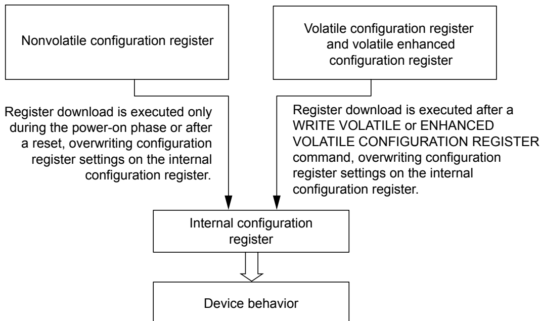
Figure 6: Internal Configuration Register
