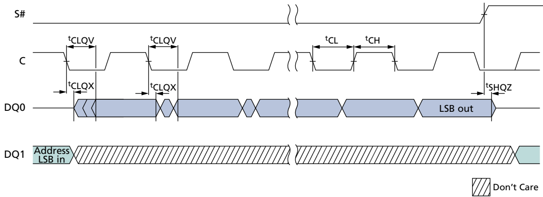
Figure 41: Output Timing
