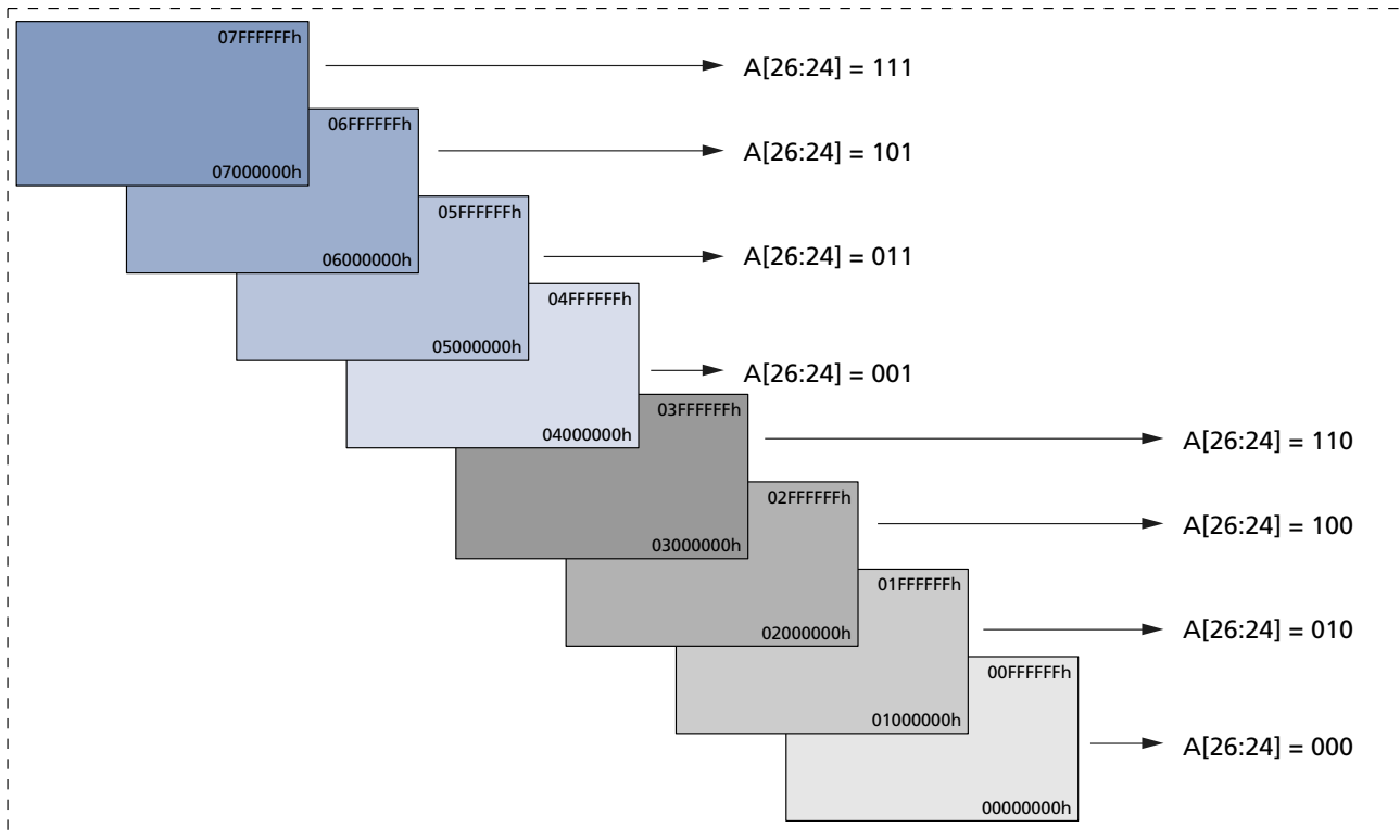
Figure 7: Upper and Lower Memory Array Segments
