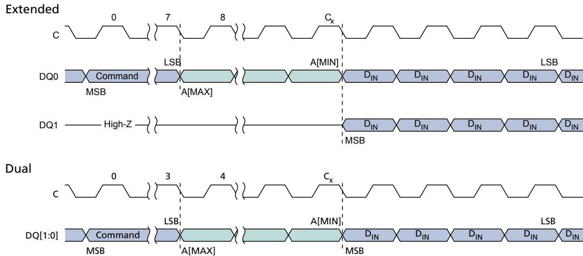
Figure 25: DUAL INPUT FAST PROGRAM Command
