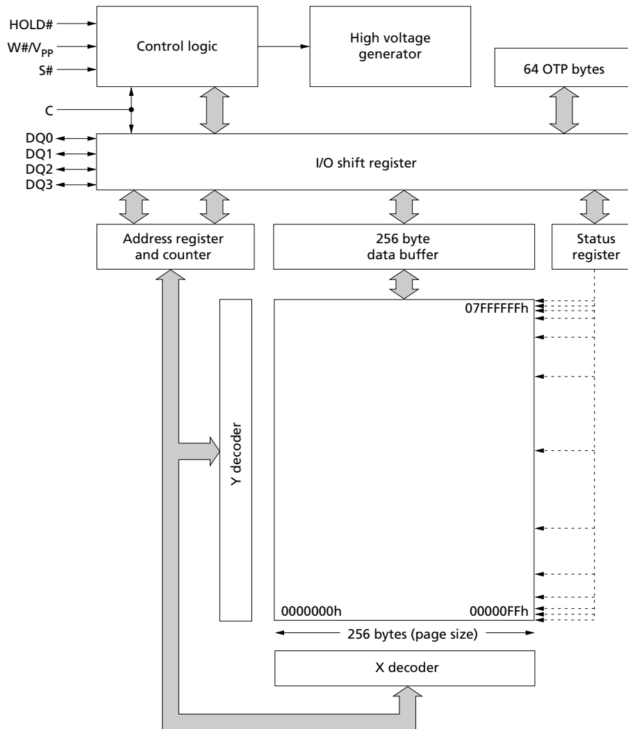
Figure 3: Block Diagram
