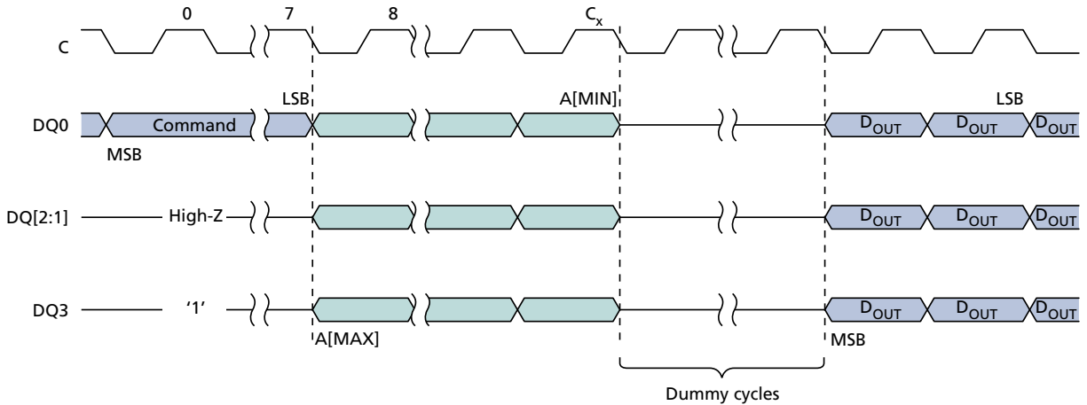
Figure 18: QUAD INPUT/OUTPUT FAST READ Command
