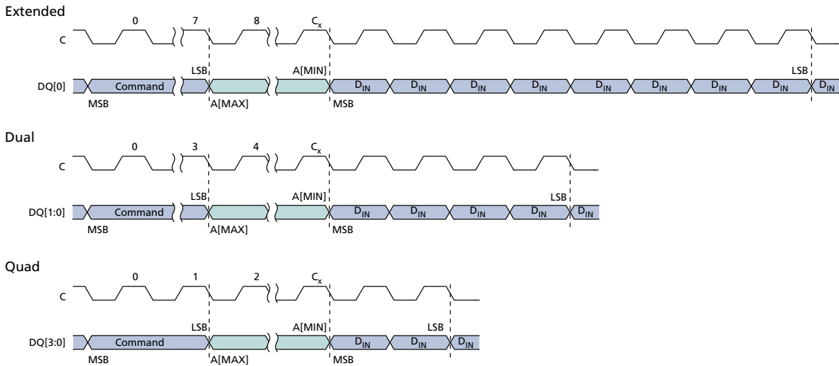
Figure 24: PAGE PROGRAM Command
