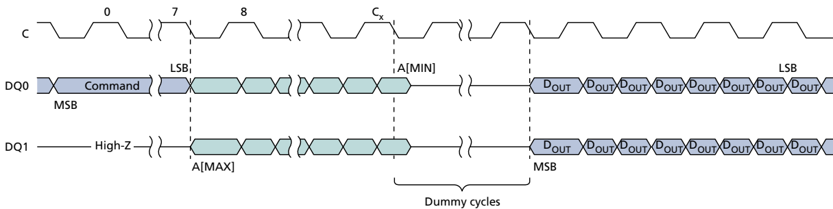
Figure 21: DUAL INPUT/OUTPUT FAST READ Command – DTR
