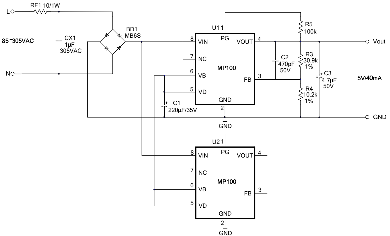
Figure 6: Paralleled Application
