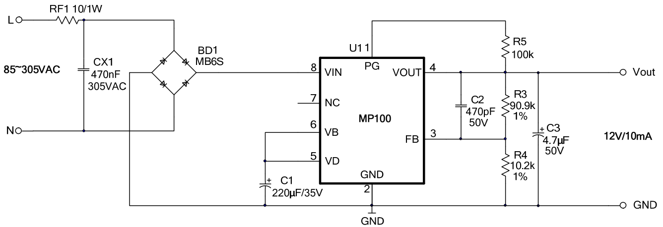
Figure 5: Typical Application
