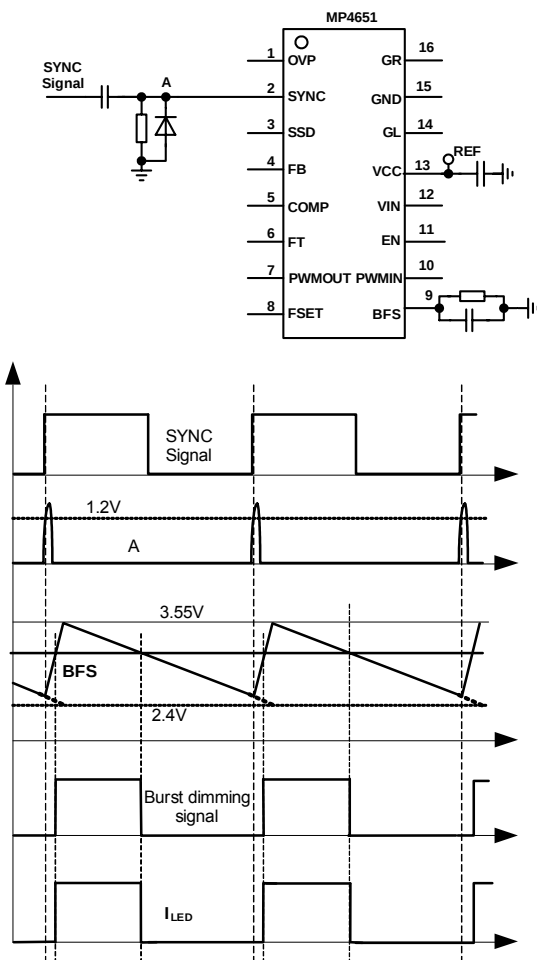
Figure 4—Synchronized DC Input Burst Dimming
