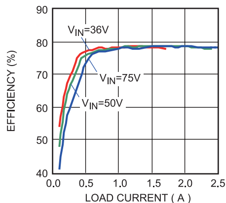
Load Efficiency
