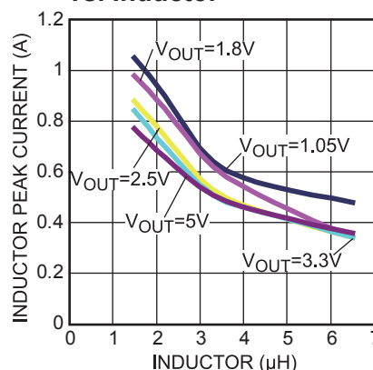
Figure5—Inductor Peak Current vs. Inductor
