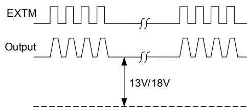
Figure 2: Tone Signal at Output
