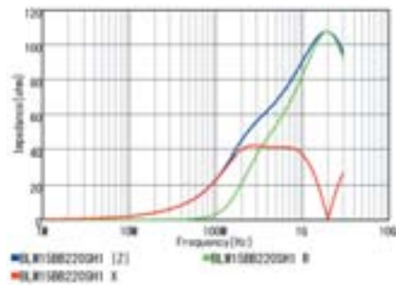
BLM15BB220SZ1/BLM15BB220SH1
