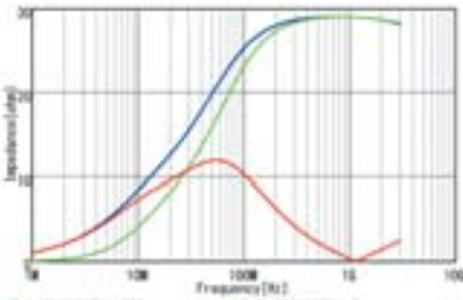
BLM18KG260TZ1/BLM18KG260TH1
