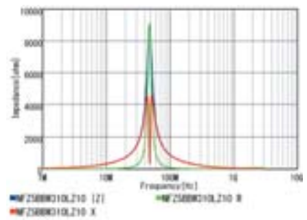
NFZ5BBW310LZ10
