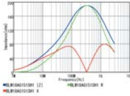
BLM18AG151SZ1/BLM18AG151SH1
