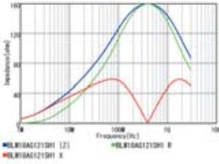
BLM18AG121SZ1/BLM18AG121SH1
