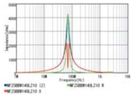
NFZ5BBW140LZ10
