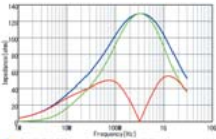
BLM18KG101TZ1/BLM18KG101TH1
