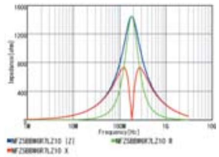
NFZ5BBW6R7LZ10
