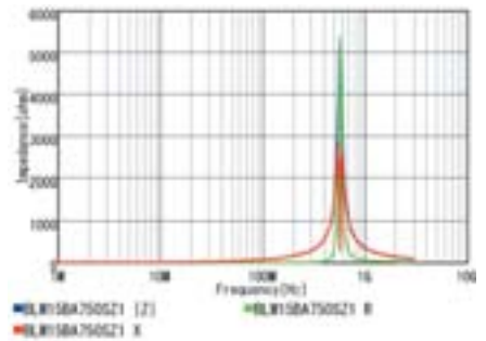
BLM15BA750SZ1
