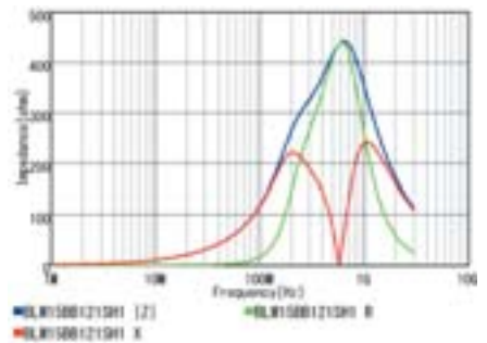
BLM15BB121SZ1/BLM15BB121SH1
