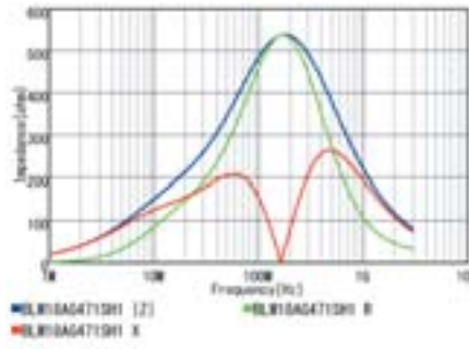
BLM18AG471SZ1/BLM18AG471SH1
