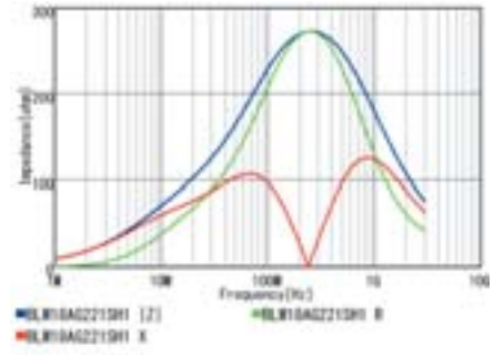
BLM18AG221SZ1/BLM18AG221SH1
