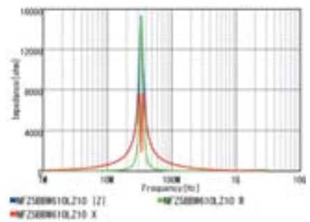
NFZ5BBW610LZ10
