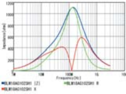
BLM18AG102SZ1/BLM18AG102SH1
