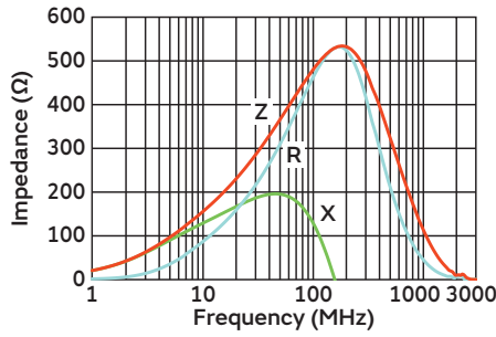
BLL18AG471A2E1H01/BLL18AG471DBE1H01
