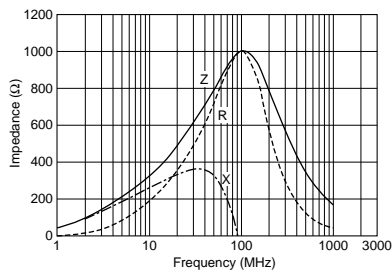
BLM18TG102TN1
