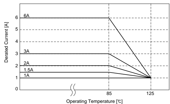
[Derating]
