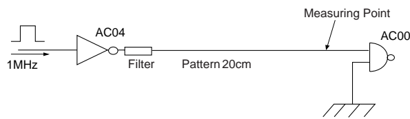
[Measuring Circuits]
