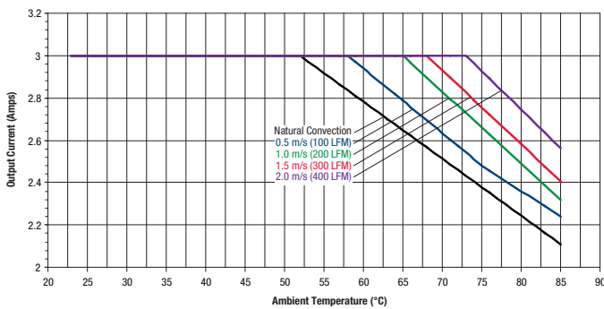
Maximum Current Temperature Derating @ sea level (VIN = 24V, transverse airflow, no baseplate)
