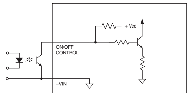
Figure 5. Driving the Negative Logic On/Off Control Pin
