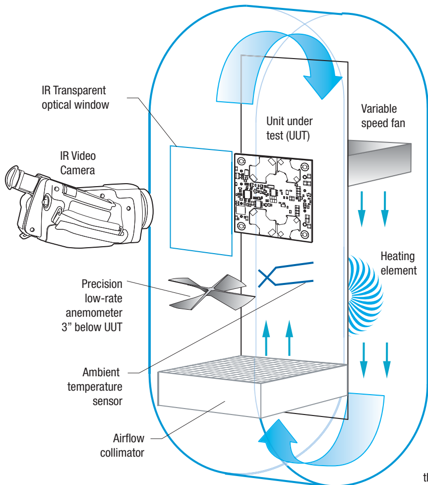
Figure 10. Vertical Wind Tunnel
