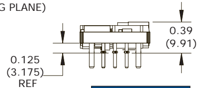
END VIEW
