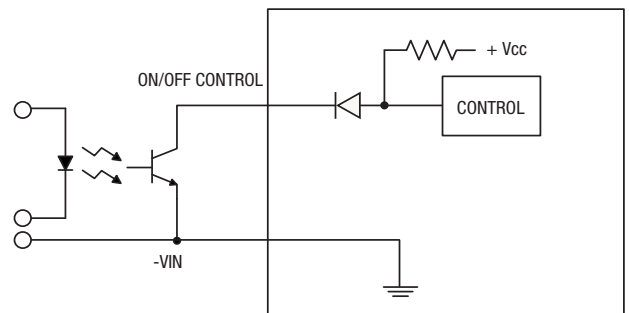
Figure 4. Driving the Positive Logic On/Off Control Pin
