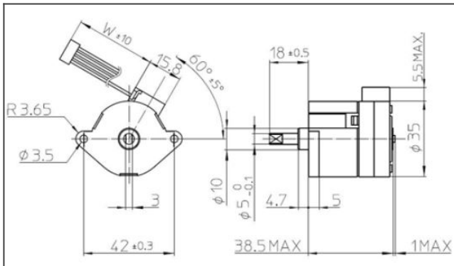
PG35S-D48 product drawing
