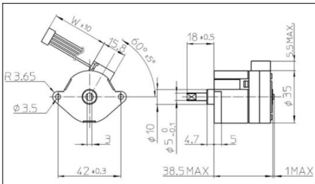
PG35S-D48-HHC2 product drawing
