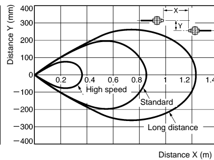
E32-T11R (Through-beam)
