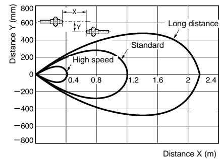
E32-T11 (Through-beam)
