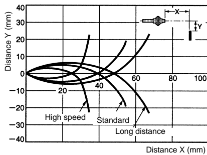
E32-DC200 (Reflective)
