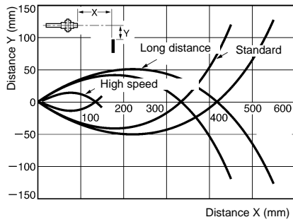
E32-DC200 (Reflective)
