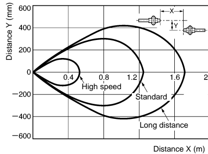
E32-TC200 (Through-beam)
