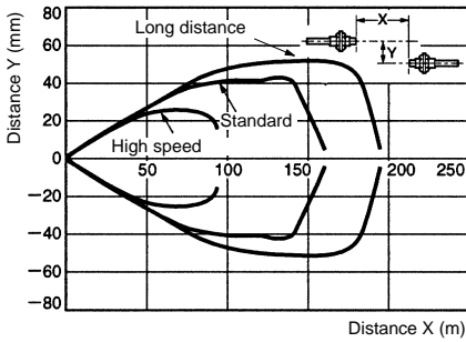
E32-TC200 (Through-beam)
