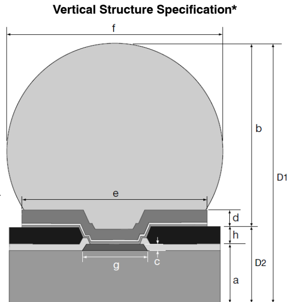
Figure 1. Sectional View
