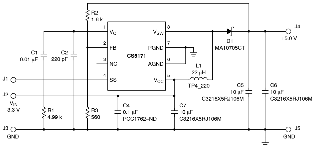
Figure 3. Schematic
