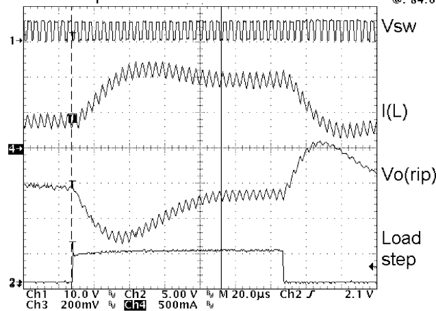
Figure 15. Transient Load
