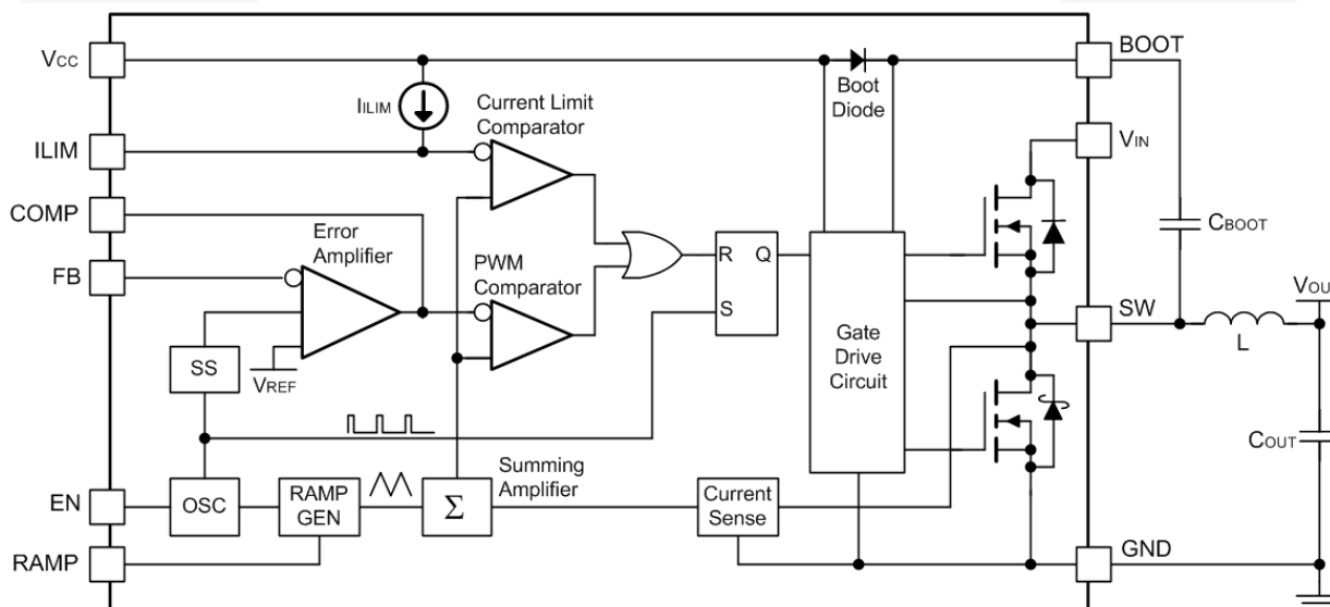
Figure 2. Block Diagram
