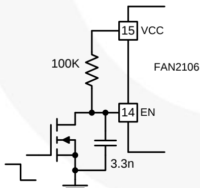
Figure 23. Enable Control with Latch Option
