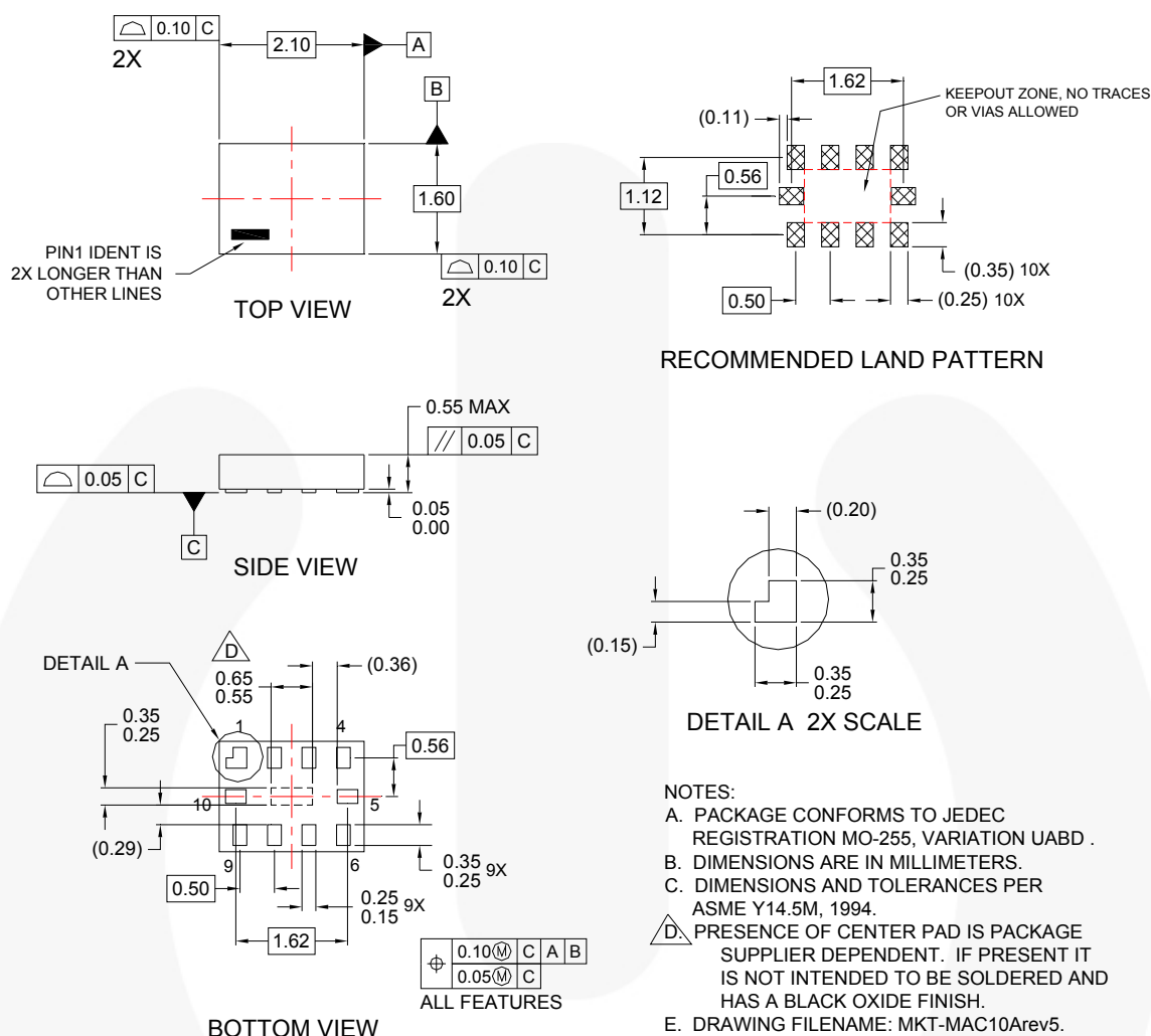
Figure 28. 10-Lead MicroPak™
