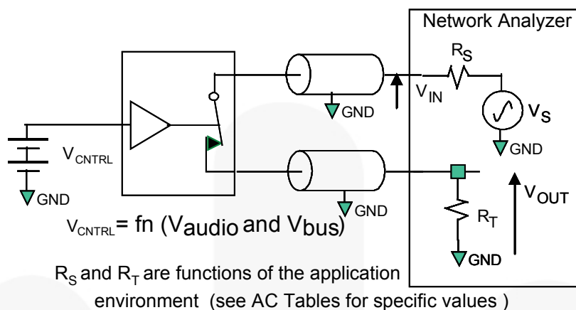
Figure 22. USB Bandwidth
