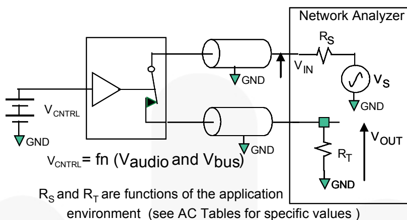
Figure 22. USB Bandwidth
