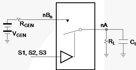
Figure 14. Charge Injection Test ( Q = \Delta V_{OUT} \cdot C_L )
