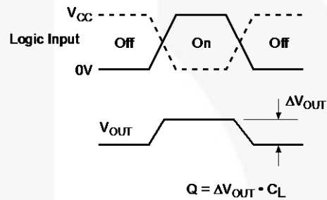
Figure 14. Charge Injection Test ( Q = \Delta V_{OUT} \cdot C_L )
