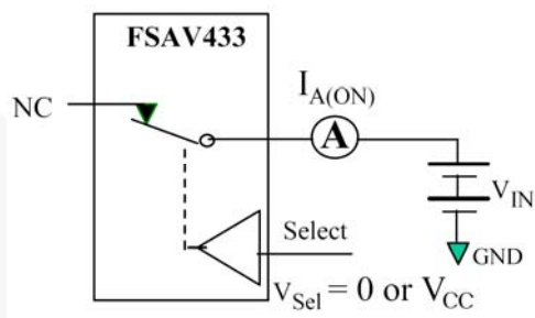
Figure 11. On Leakage
