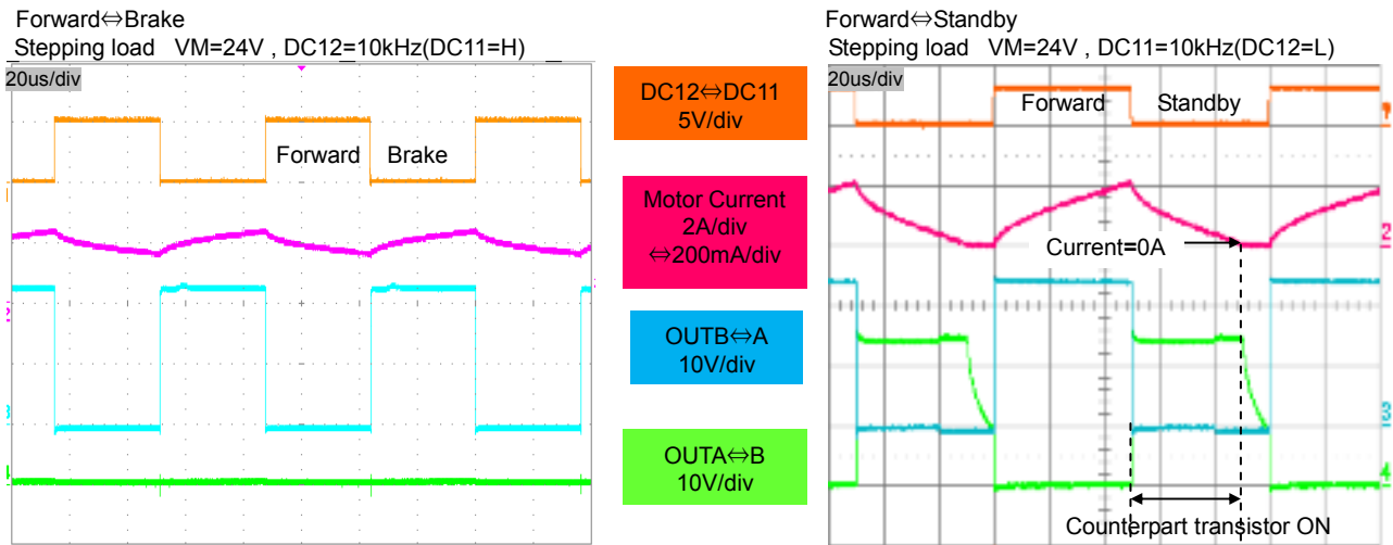
Figure 14. Stepping load control waveform
