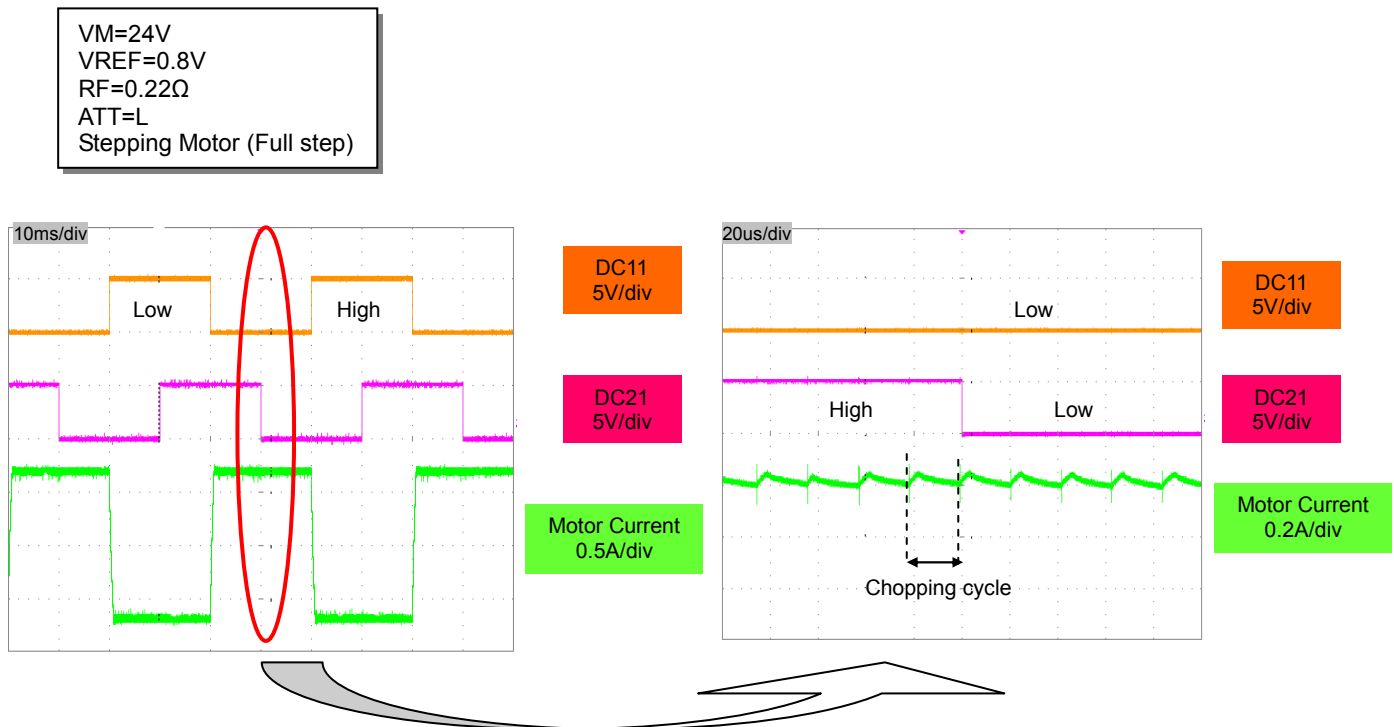
Figure 18. Setting constant-current control waveform (Stepping motor)
