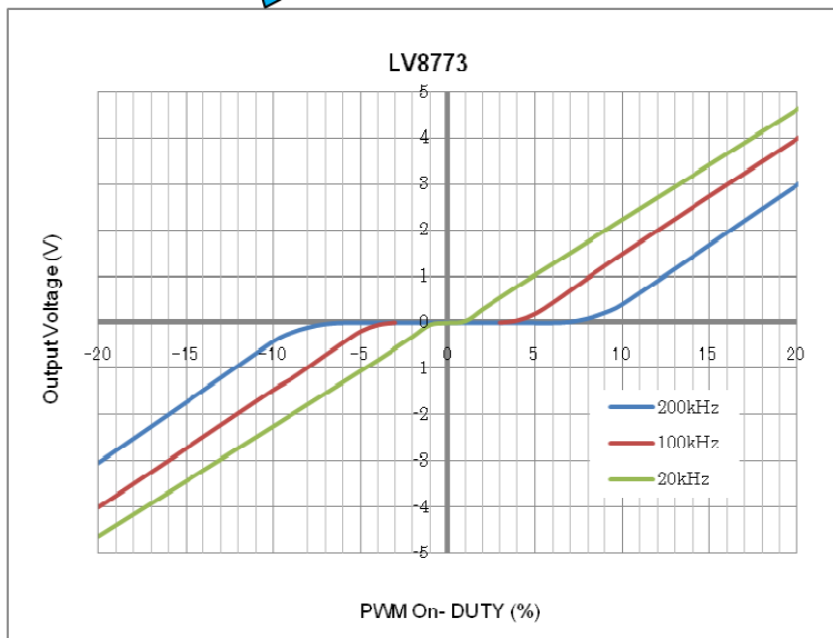
Figure 16. PWM control characteristic
