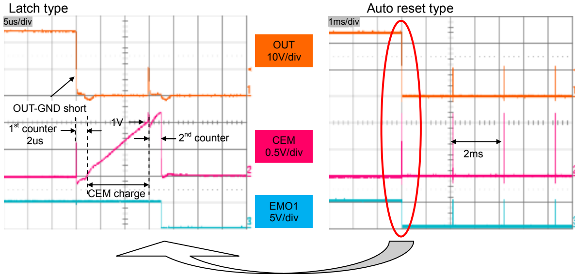
Figure 20. CEM operation waveform
