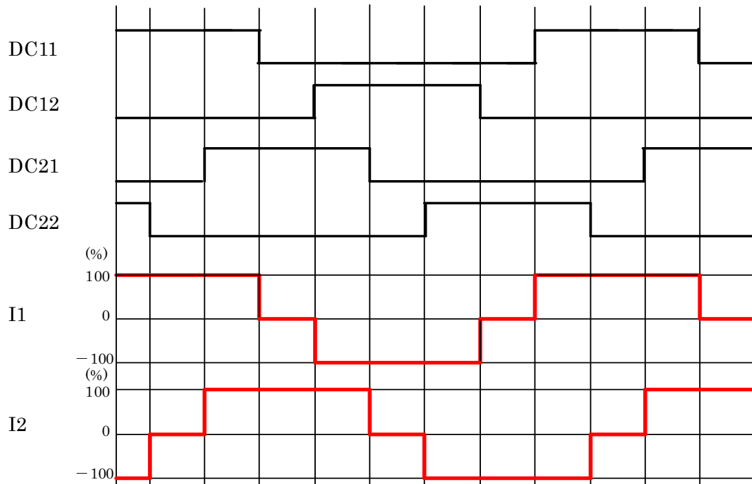
Half step (CW mode)
