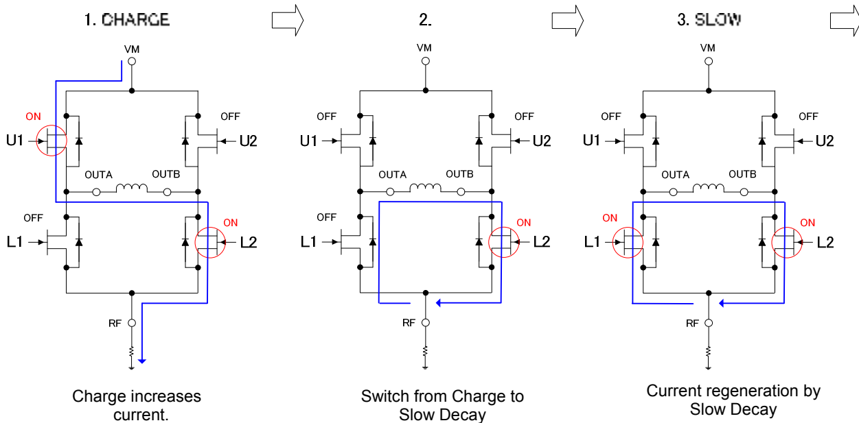
Figure 15. Switching operation
