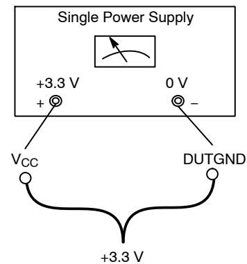
Figure 8. Single Power Supply Connections
