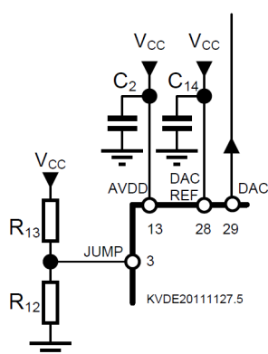
Figure 12. DAC Interface
