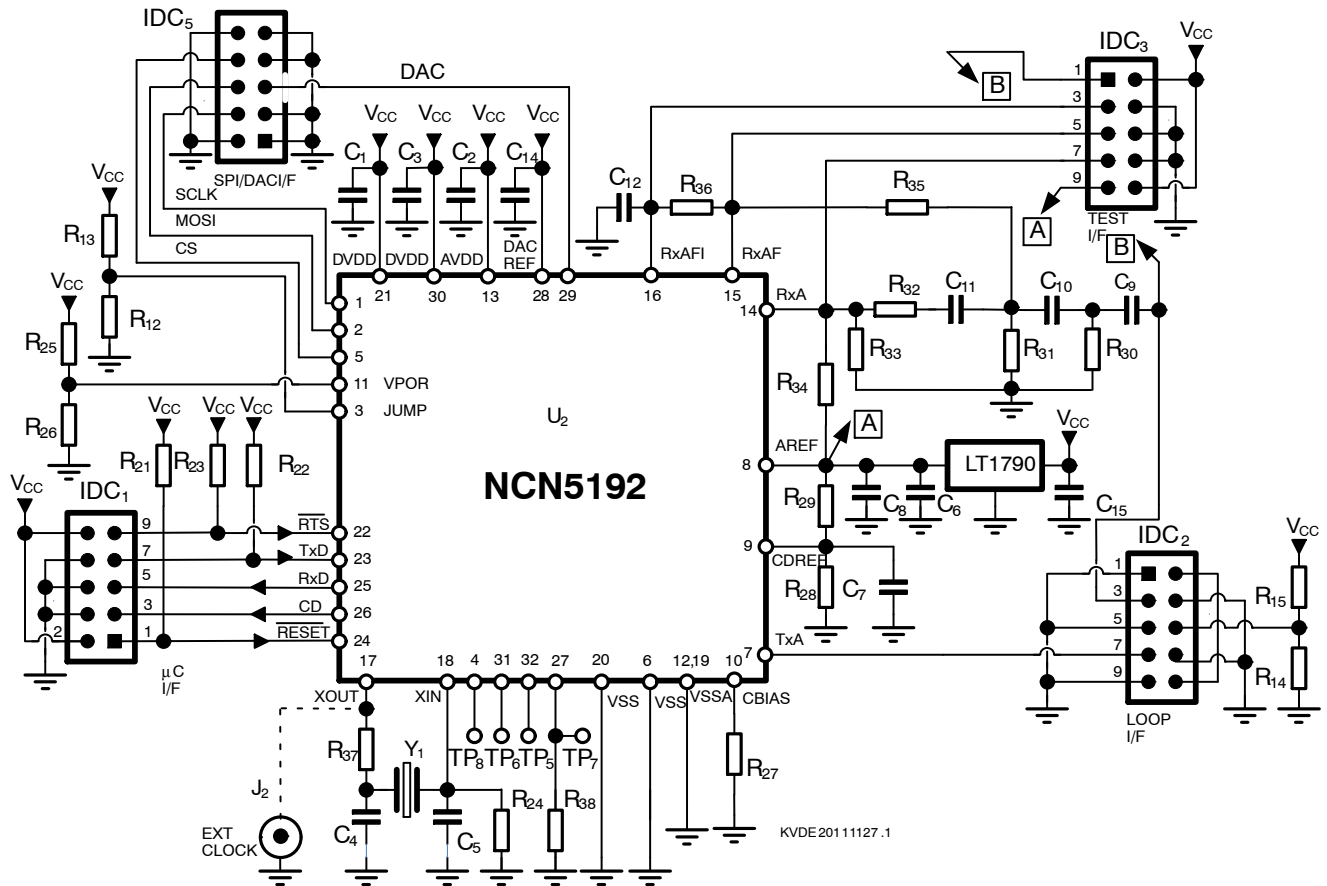
Figure 2. NCN5192NGEVB Schematic
