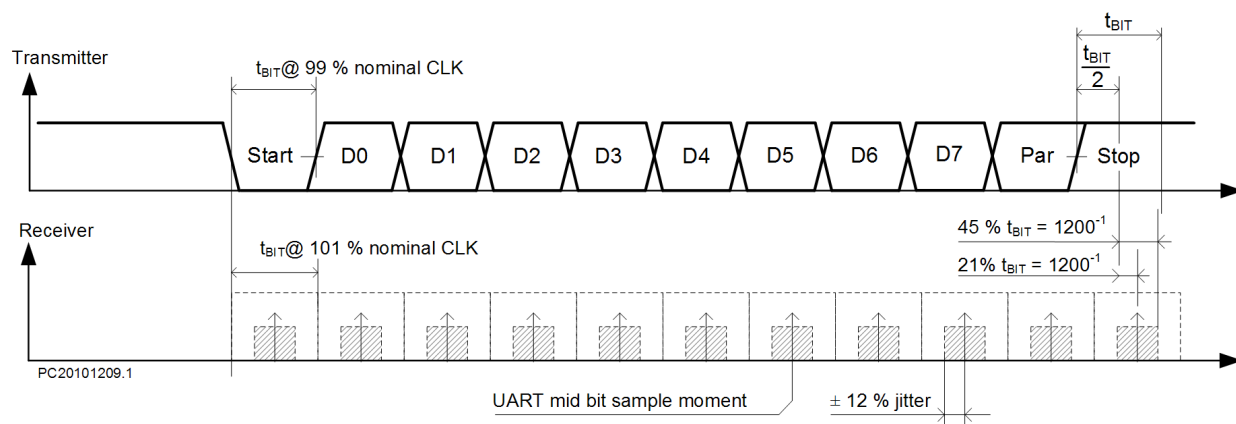
Figure 10. Clock Skew
