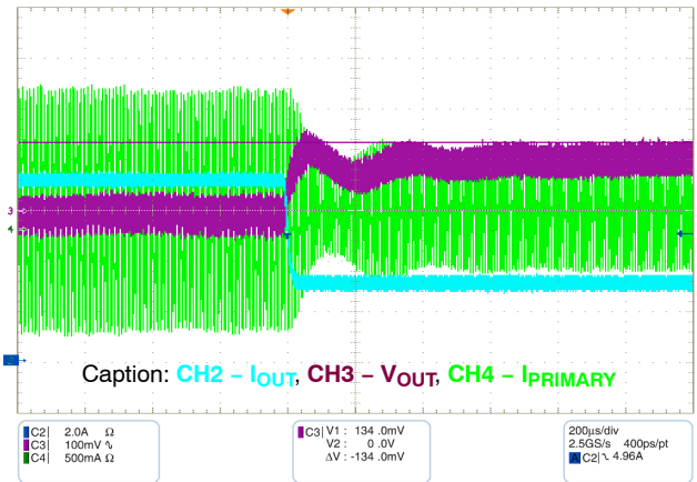
Figure 18. Transition Response - Load Step from 7 to 3 A
