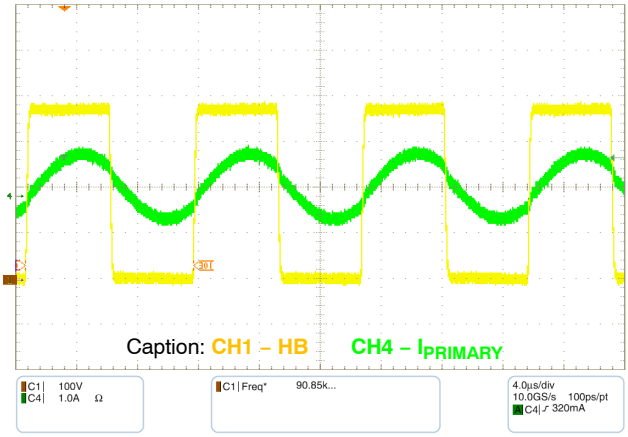
Figure 14. Steady Stage - I LOAD = 4 A
