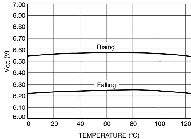
Figure 4. V_{CC} UVLO
