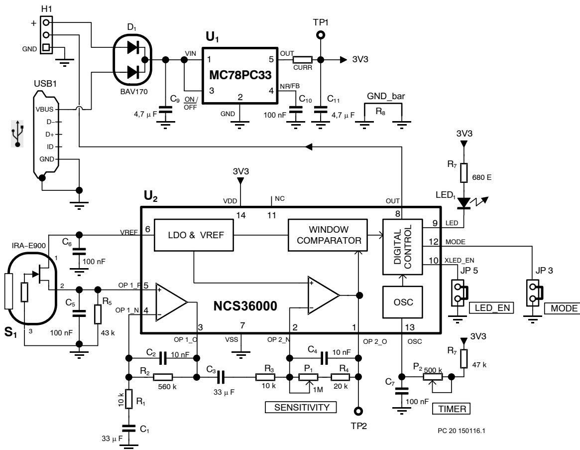
Figure 3. Schematic Diagram
