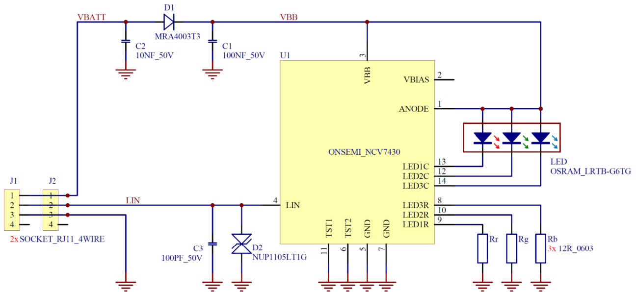
Figure 22. NCV7430 Schematic
