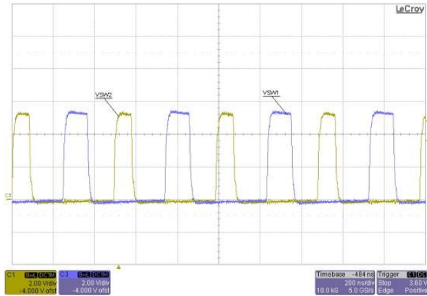
Figure 2. Normal Operation
