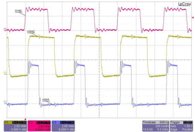
Figure 3. Synchronization
