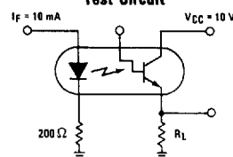
Test Circuit
