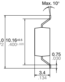
Surface mount terminal type
