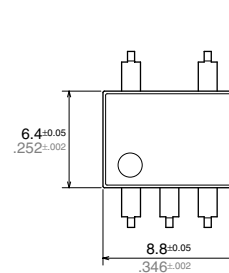
Surface mount terminal type
