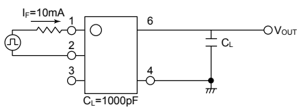
***Turn on/Turn off time measurement circuit APV1122(A)
