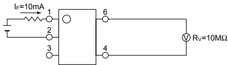
*Drop-out voltage measurement circuit APV1122(A)
