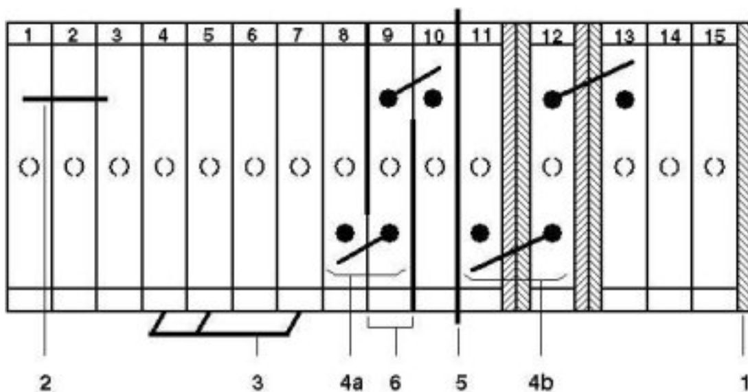
Circuit diagram
