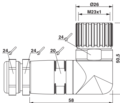
Dimensional drawing
