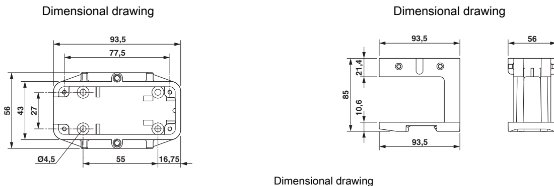
Dimensional drawing top view
