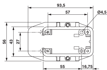
Dimensional drawing top view
