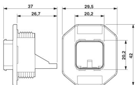
Push-Pull panel mounting frame, Freenet system, IP67
